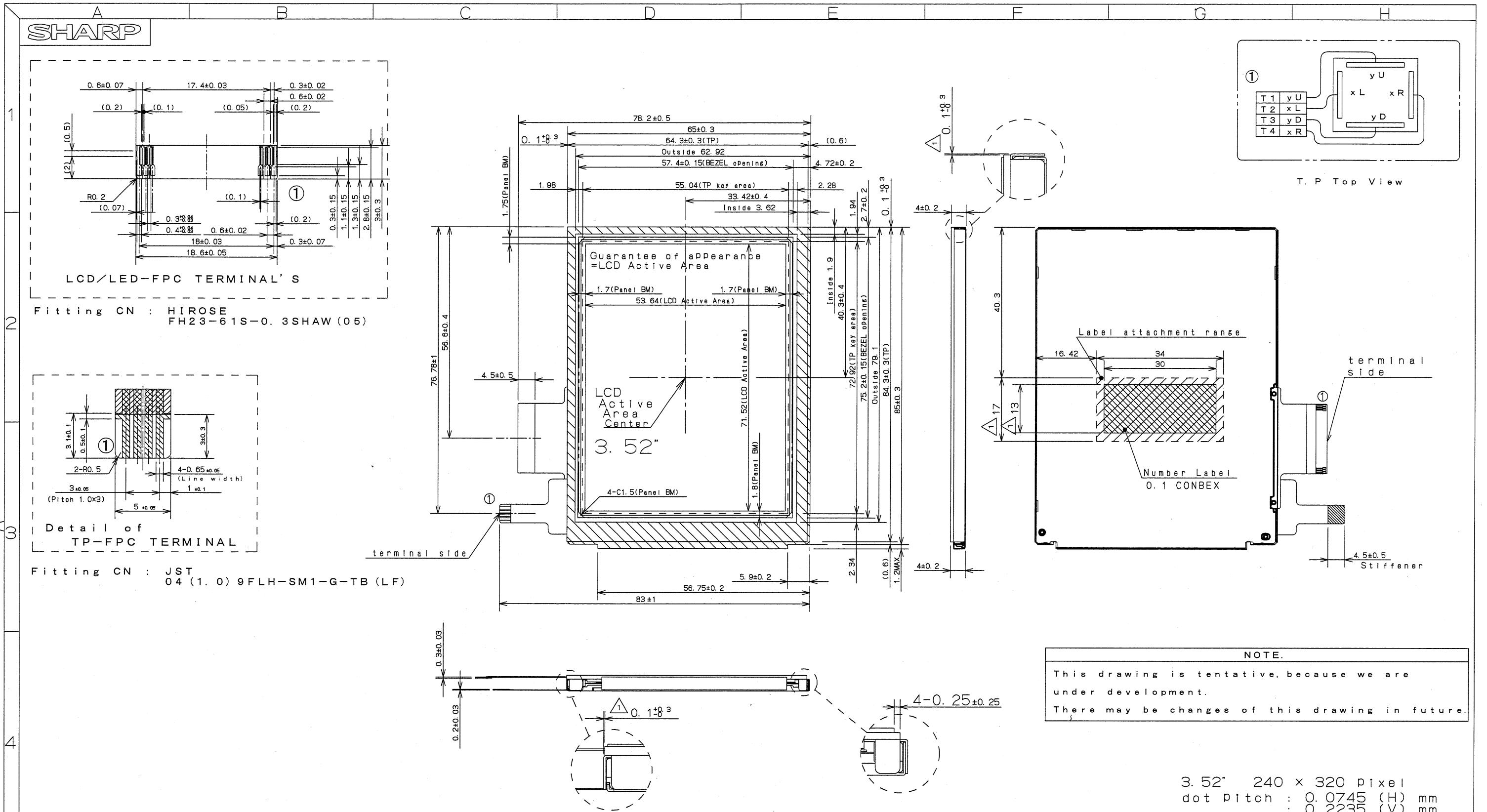
Fig. 1 Outline Dimension
