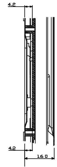
SECTION D-D SCALE 2,000
