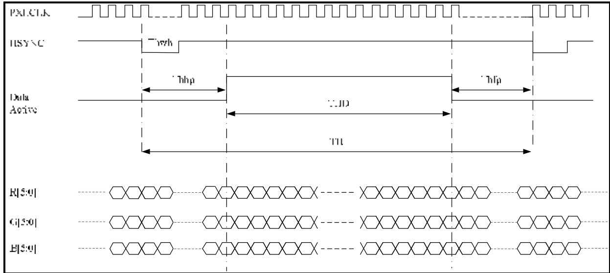
Horizontal Input Data Timing Diagram
