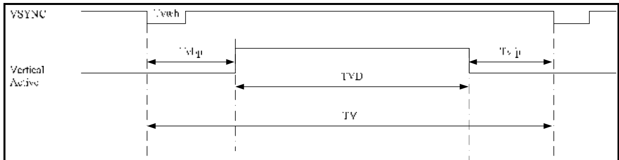
Vertical Input Data Timing Diagram
