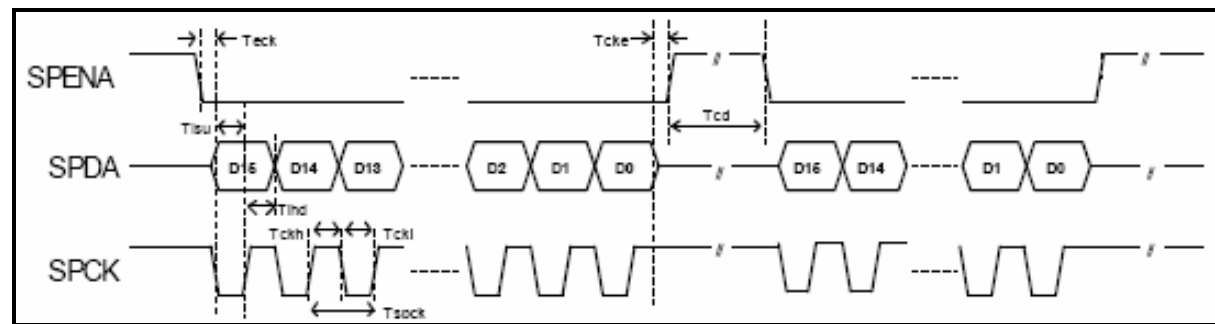
3-wire Timing Diagram
