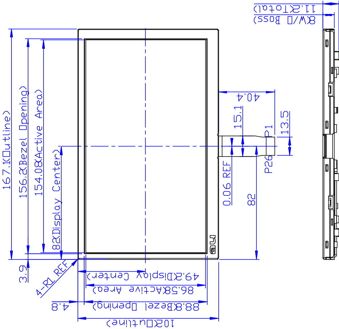
Fig.1-(a) Outline dimension of TFT-LCD module(Front side)
