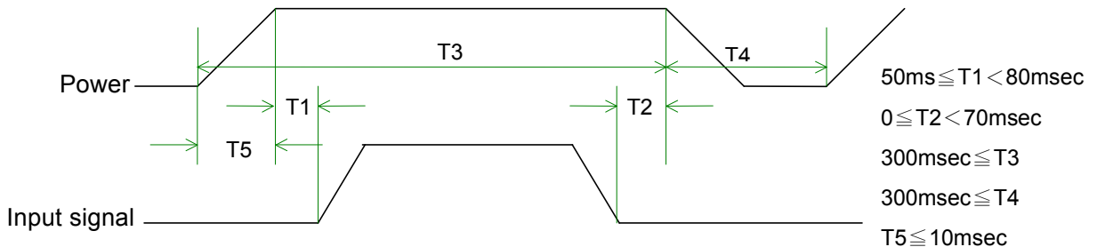
Sequence of Power-on/off and signal-on/off
