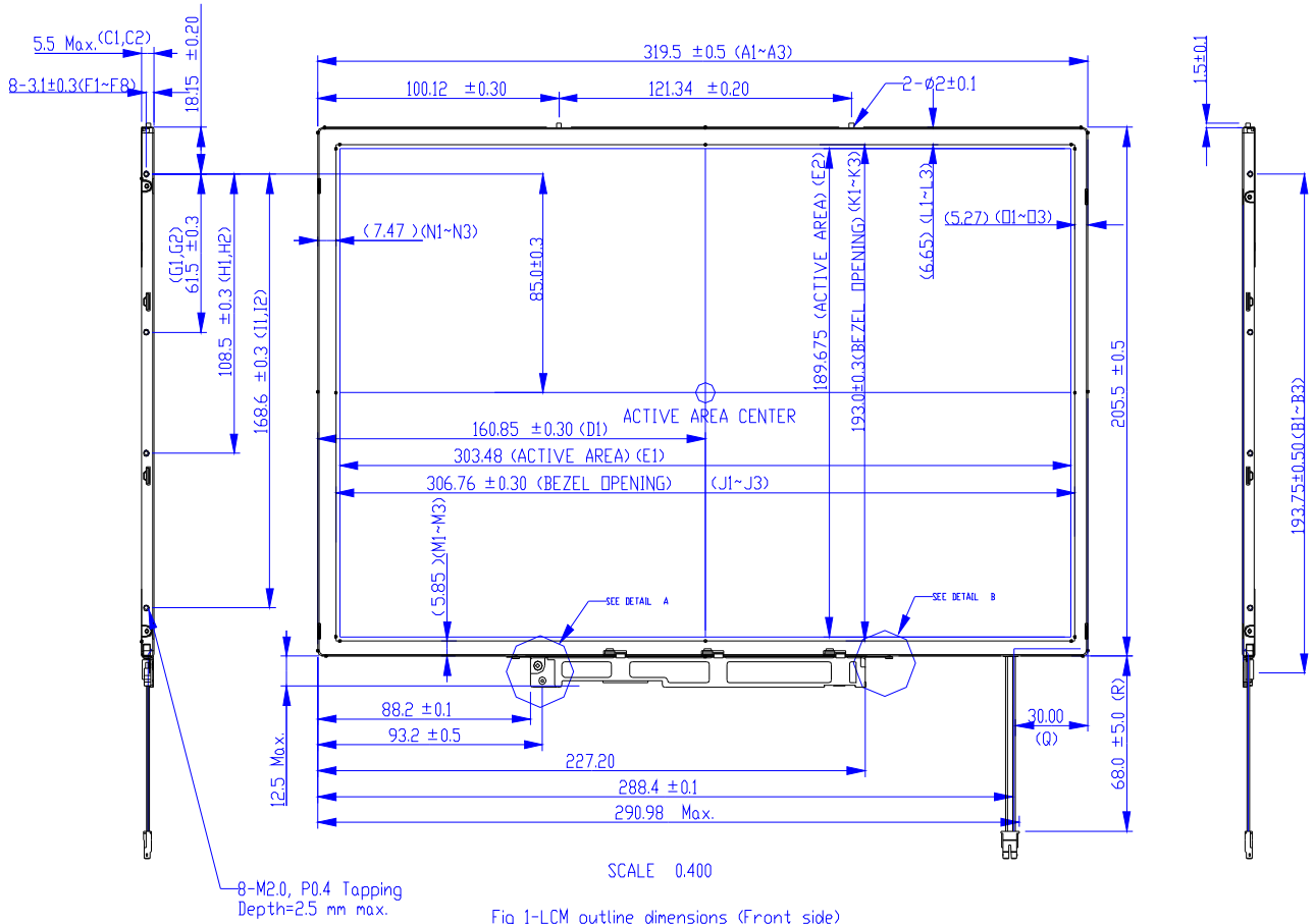
Fig 1-LCM outline dimensions (Front side)
