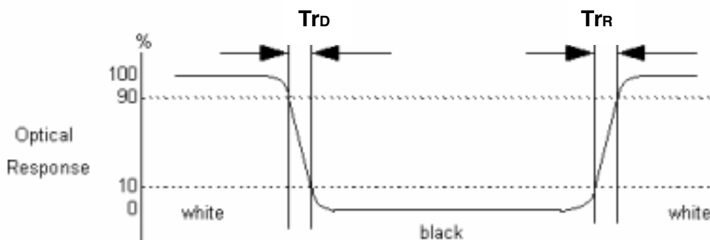
Fig.4-3 Response time
