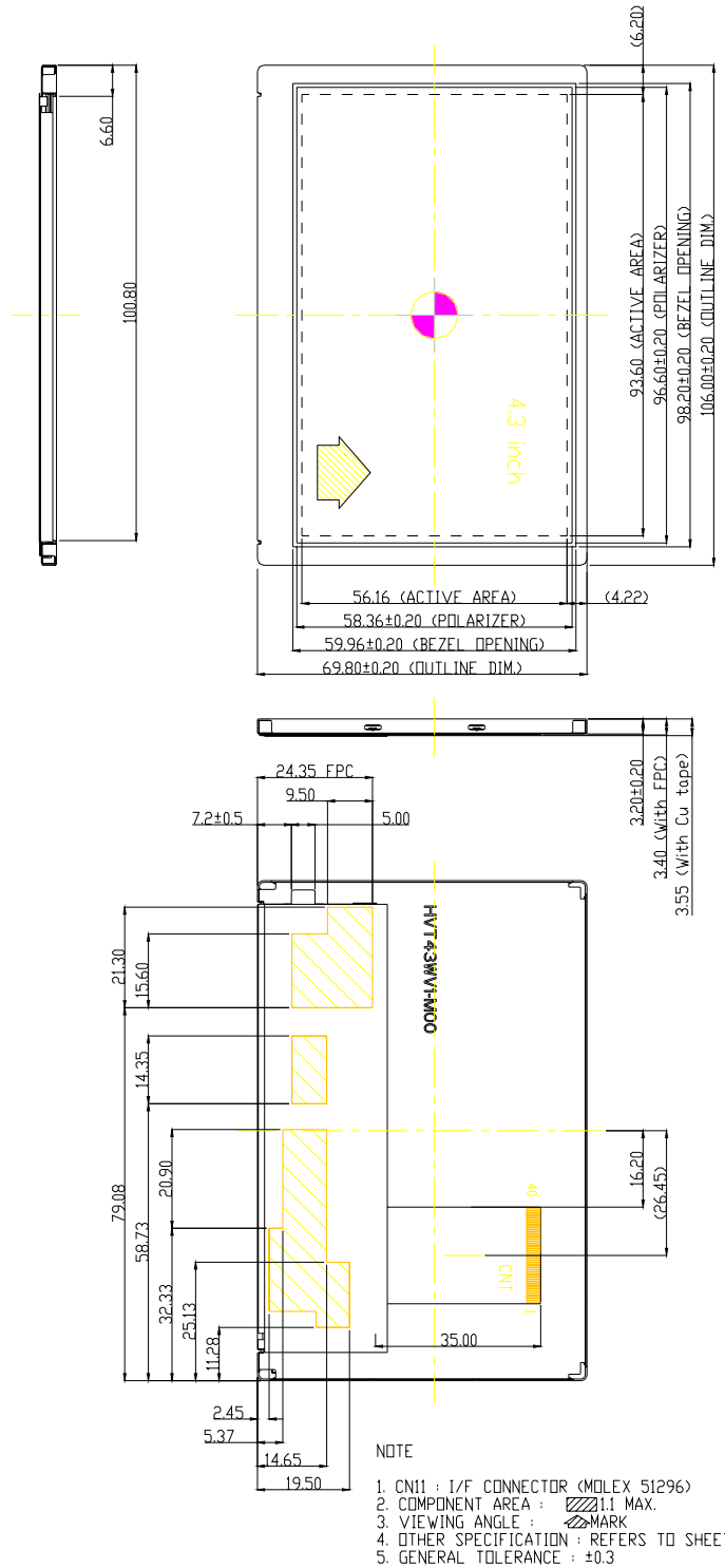
Figure 4. TFT-LCD Module Outline Dimensions
