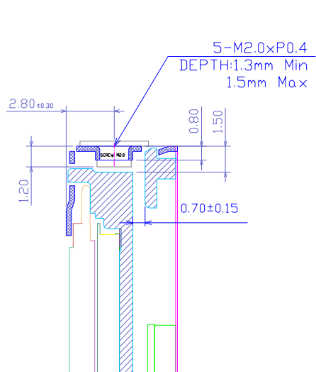
SECTION A-A(S:5/1)
