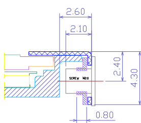
SECTION D-D(S:5/1)
