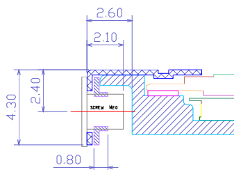
SECTION C-C(S:5/1)
