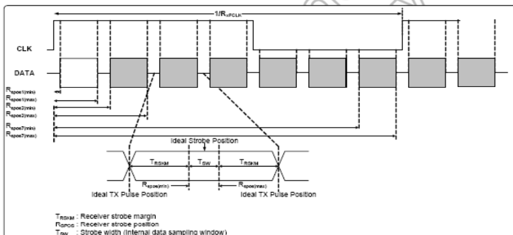
Figure 10.1: LVDS figure
