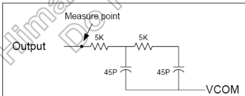
Figure 11.3: Output load condition
