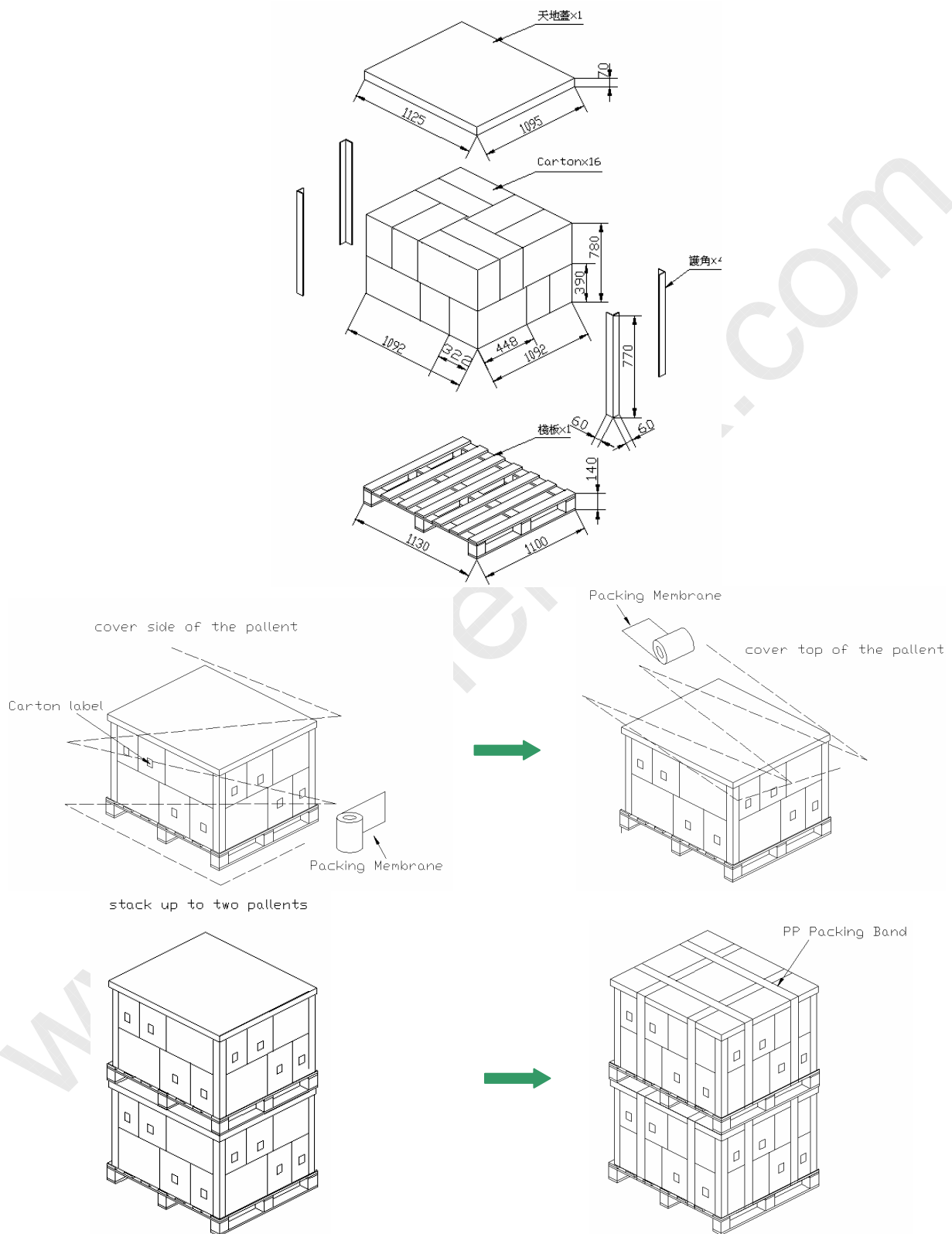
Figure. 7-2 Packing method
