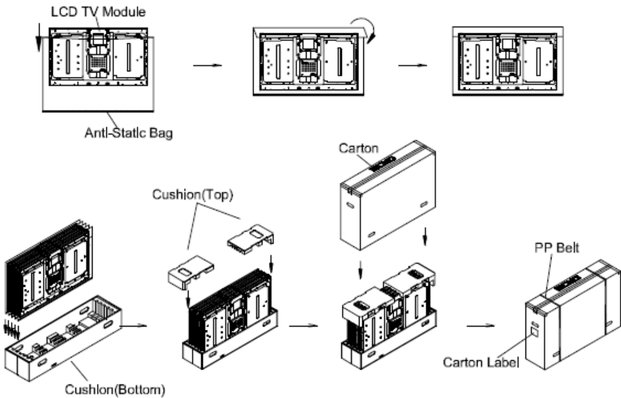
Figure.9-1 packing method
