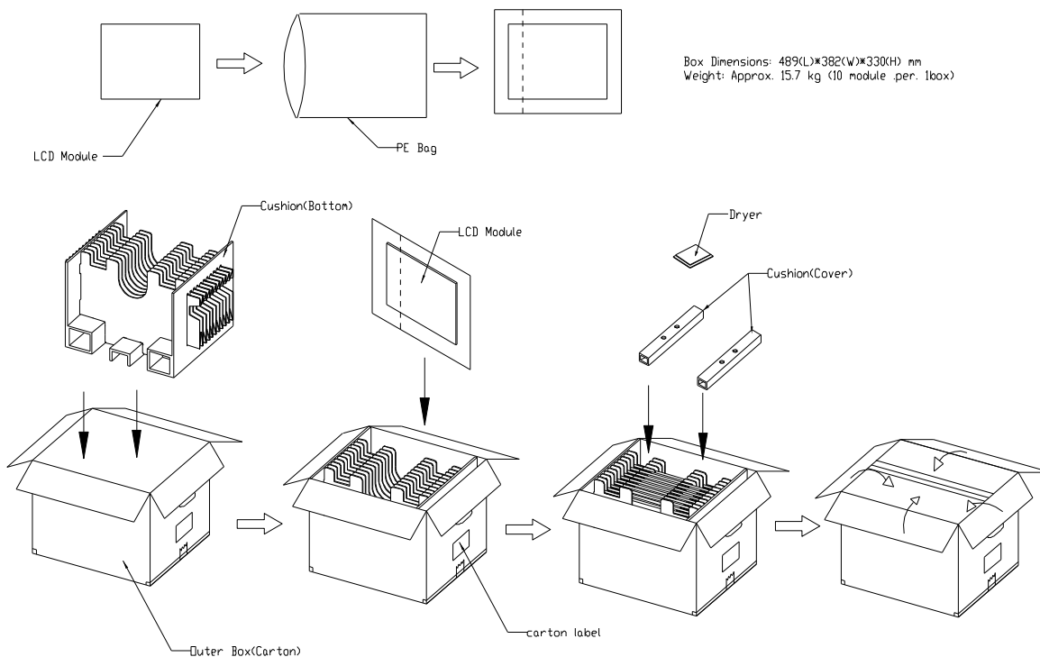
Figure. 8-1 Packing method
