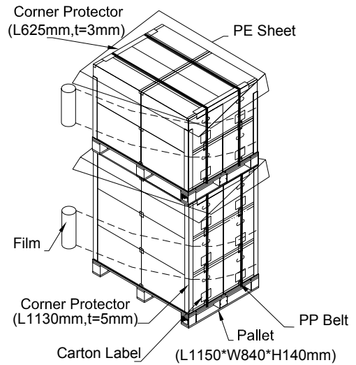
Figure. 8-2 Packing method
