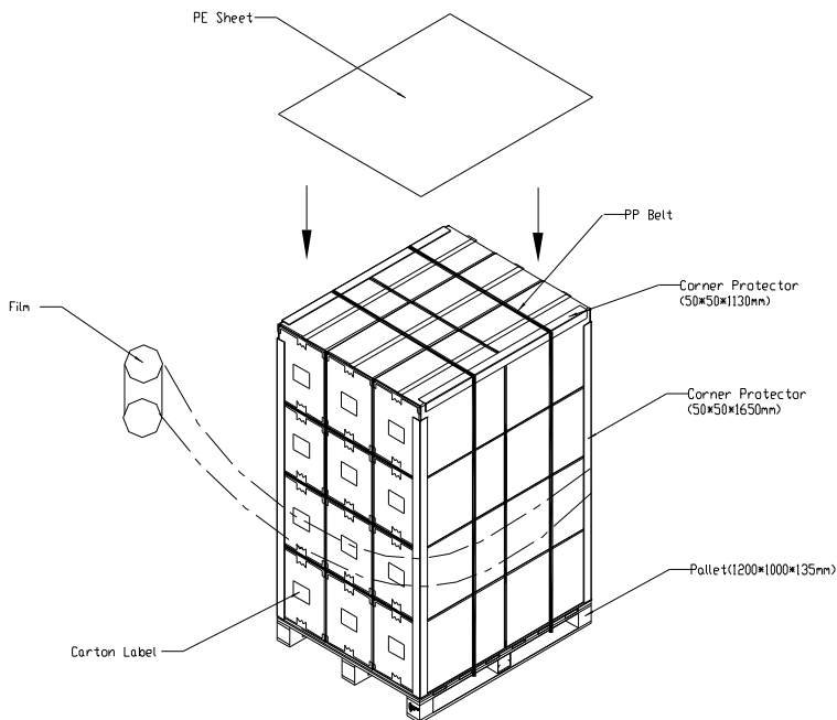
Figure. 8-2 Packing method
