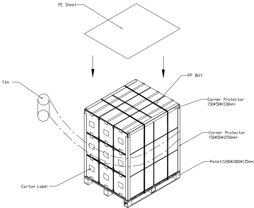
Figure. 8-3 Packing method
