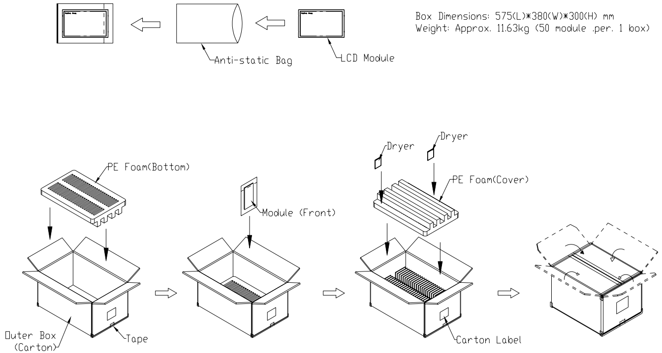
Figure. 9-1 Packing method
