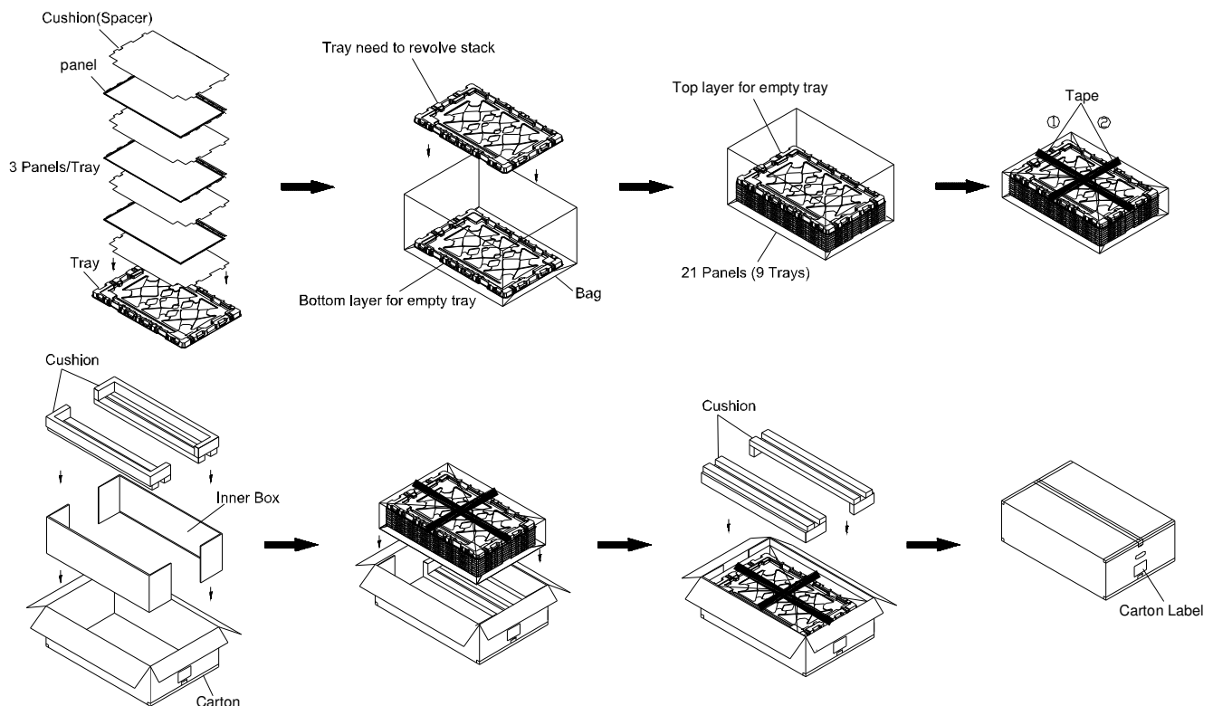
Figure.9-1 packing method
