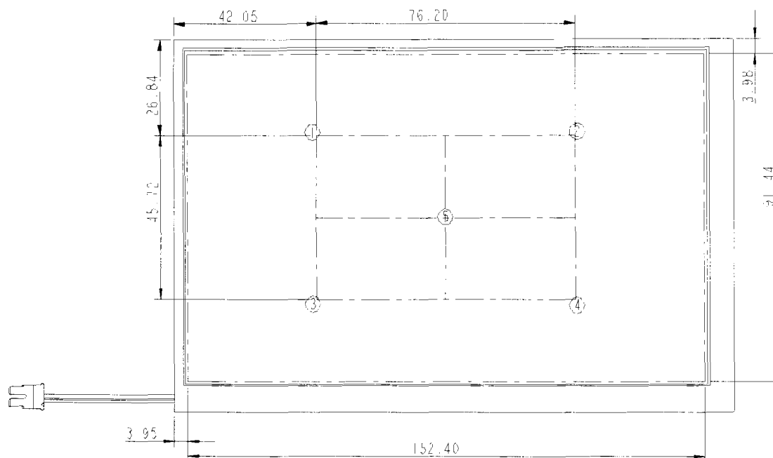
Fig.1 Measuring point
