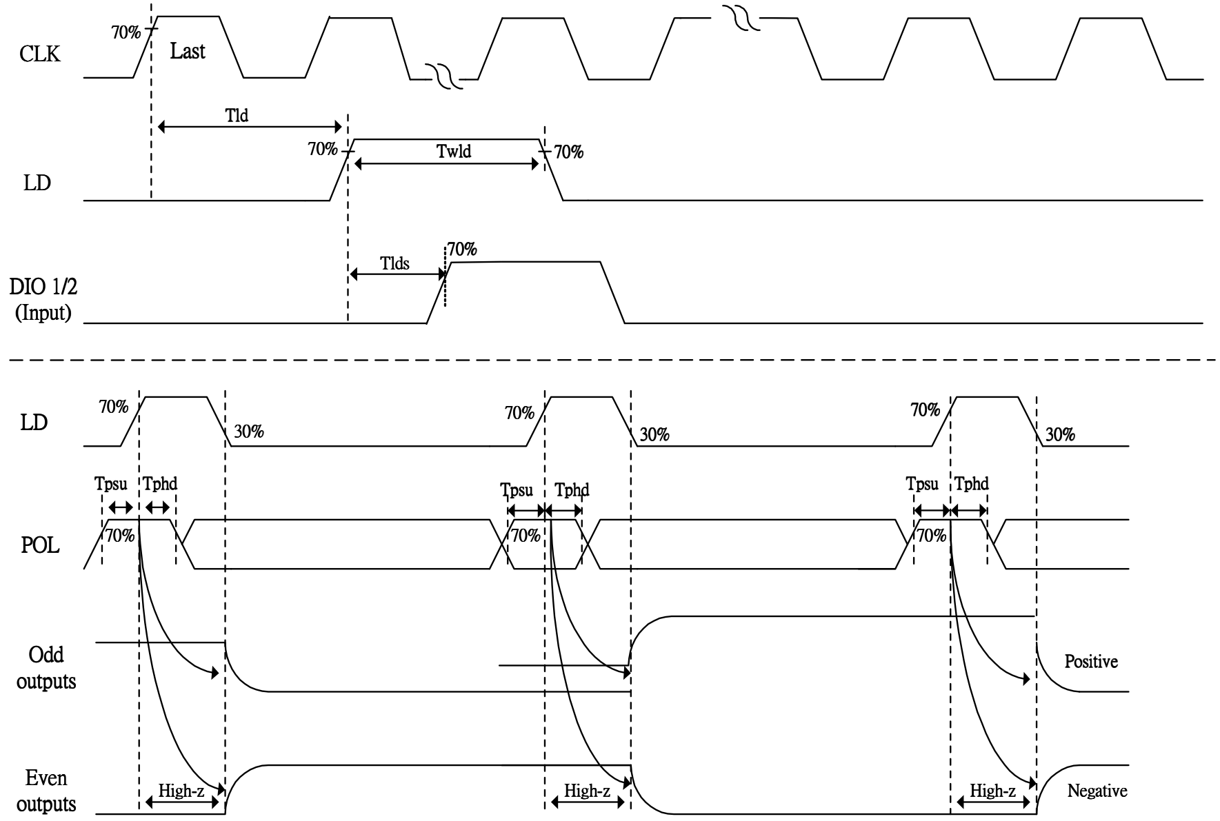
Fig. 11-2 Horizontal timing(2)
