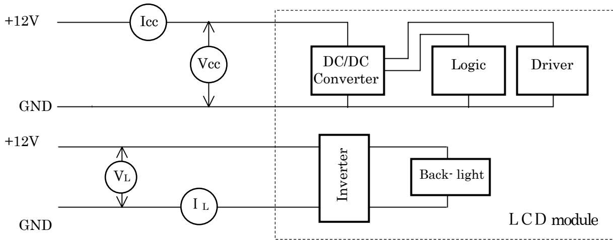
Fig.8-1. Measurement Circuit
