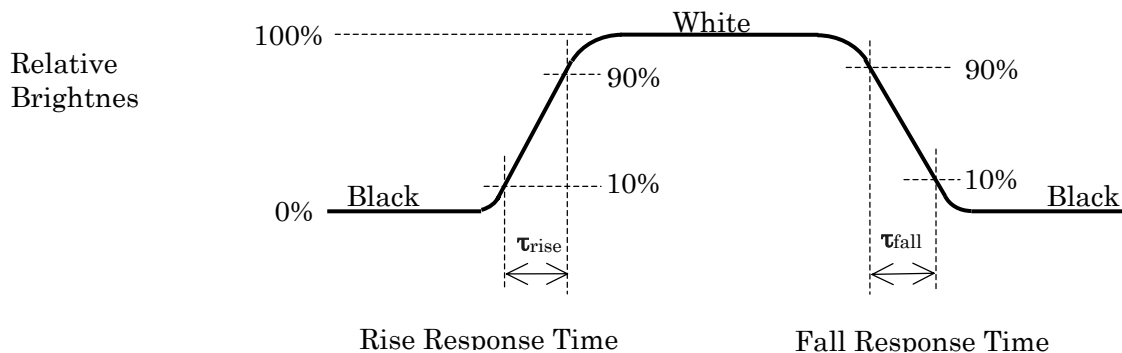
Figure 9-4 Definition of Response Time
