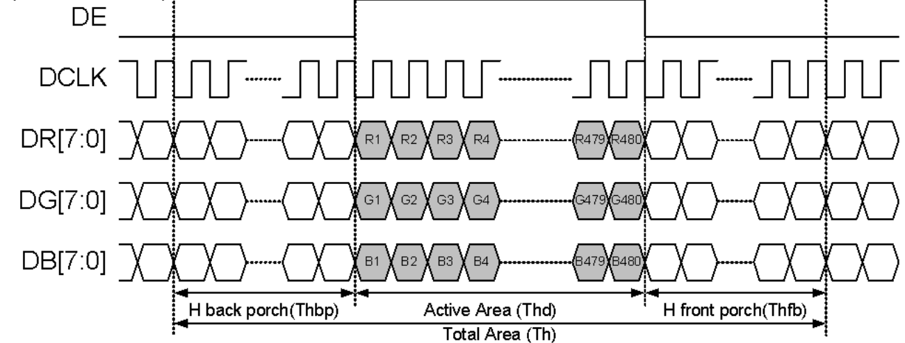
Parallel Mode Horizontal display timing (DE Mode only)
