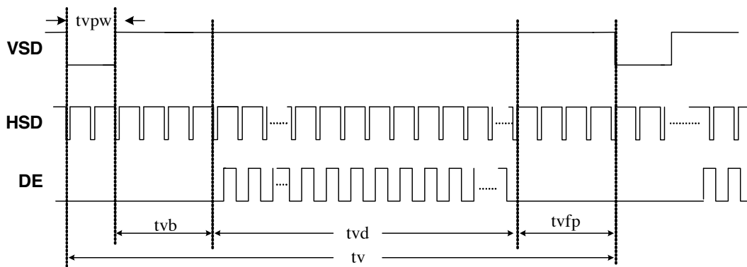
Vertical timing
