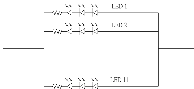
LED Light Bar Circuit
