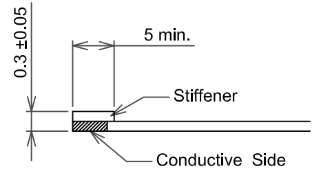
Recommended design rule for CN1 FPC
