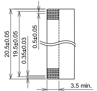
CN2 Detail
