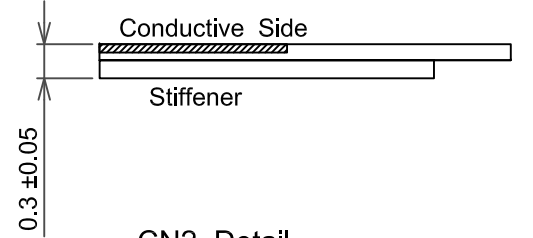
CN2 Detail
