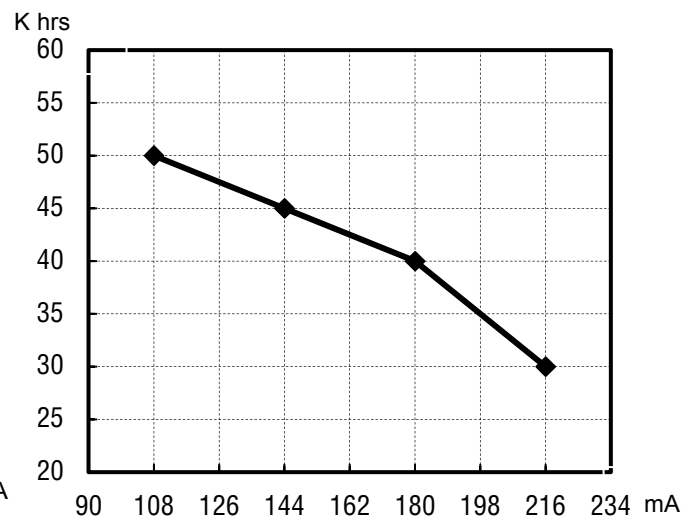
Fig 5.3 LED Current v.s. Lifetime
