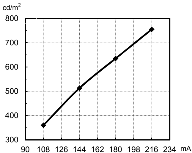
Fig 5.2 LED Current v.s. Brightness
