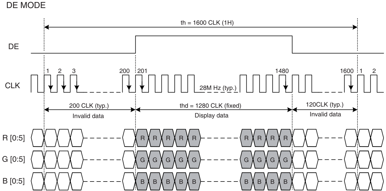
Fig. 9.3 Horizontal Timing of DE Mode
