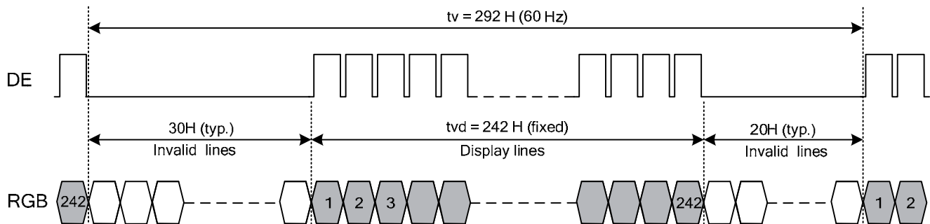
Fig. 9.4 Vertical Timing of DE Mode
