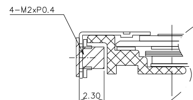
SECTION F-F
