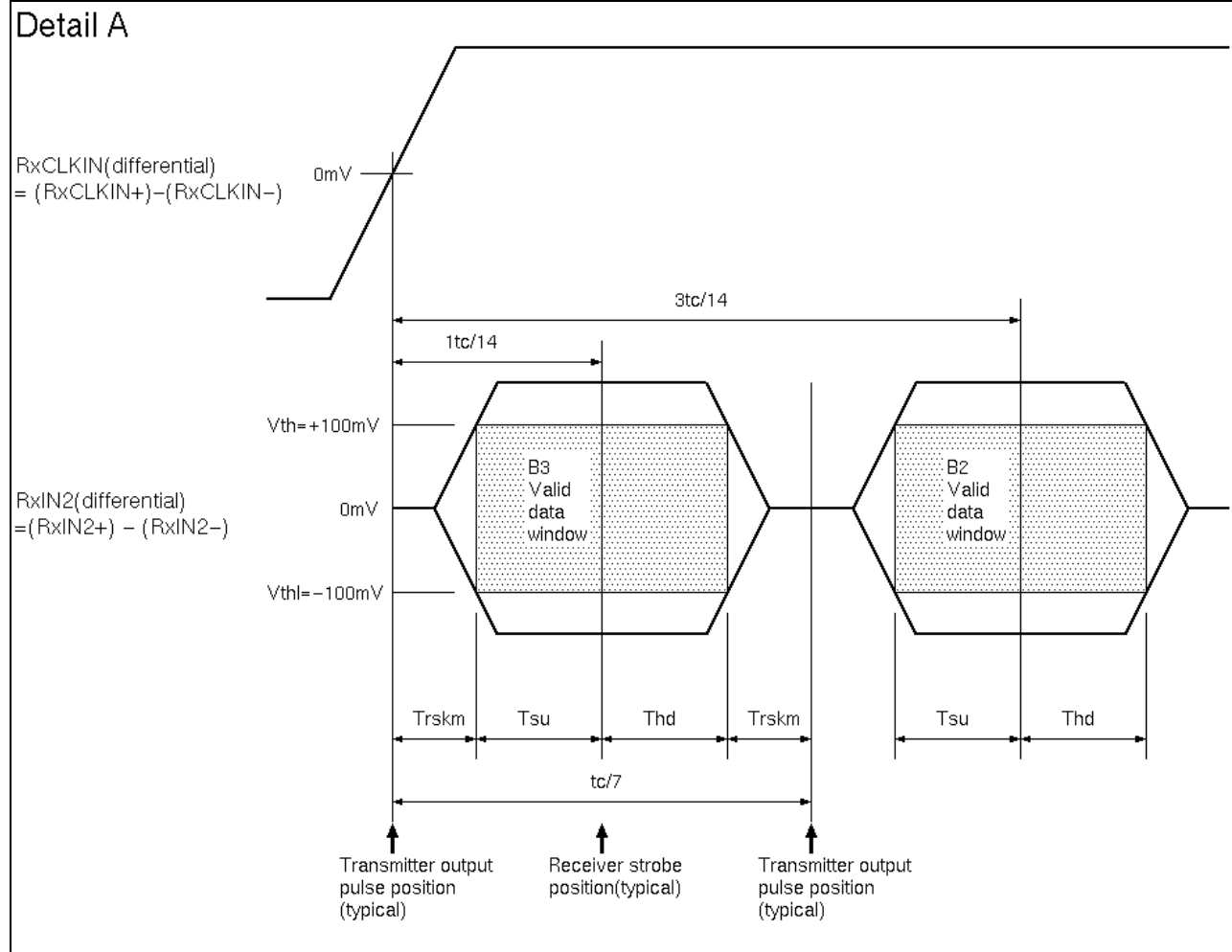
Figure . Timing Definition(detail A)
