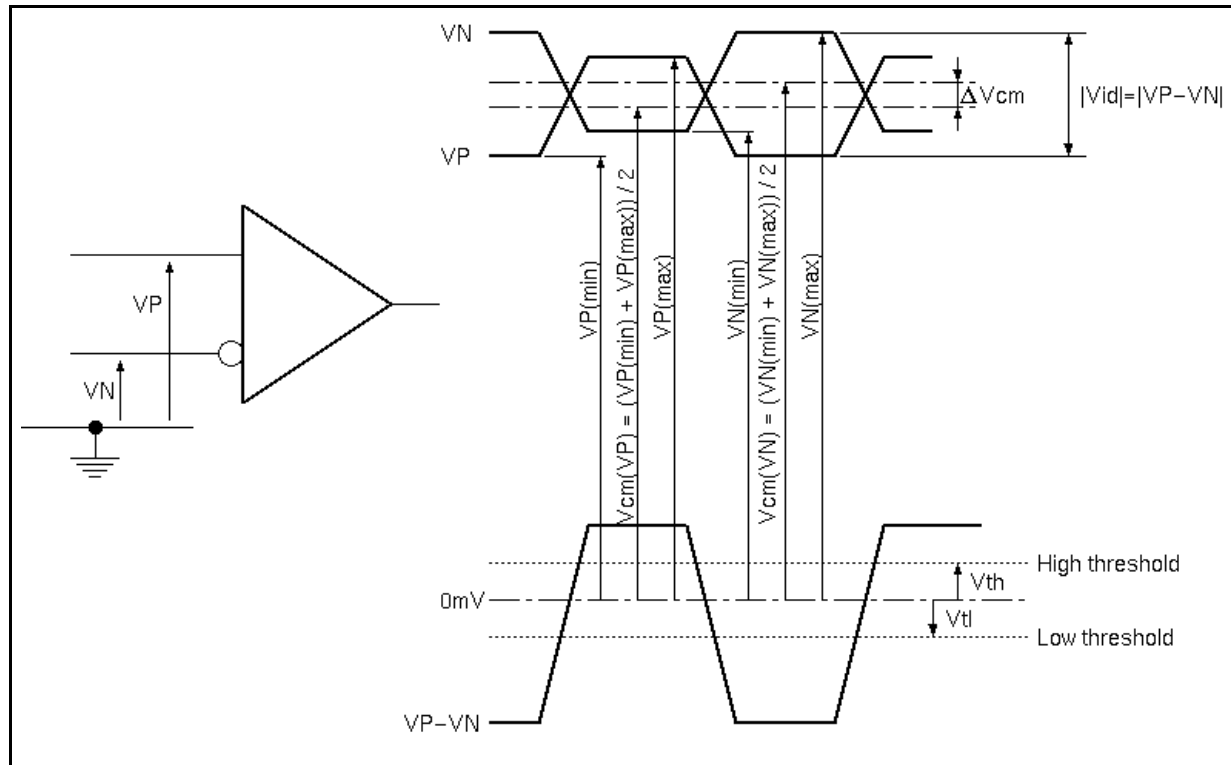
Figure. Voltage Definitions
