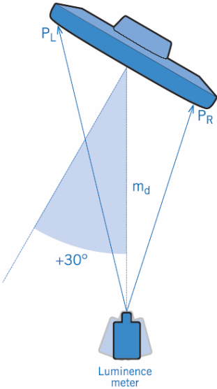
Figure2: Top view of test set-up when the screen is rotated ±30 degrees. The +rotation is defined clockwise.
