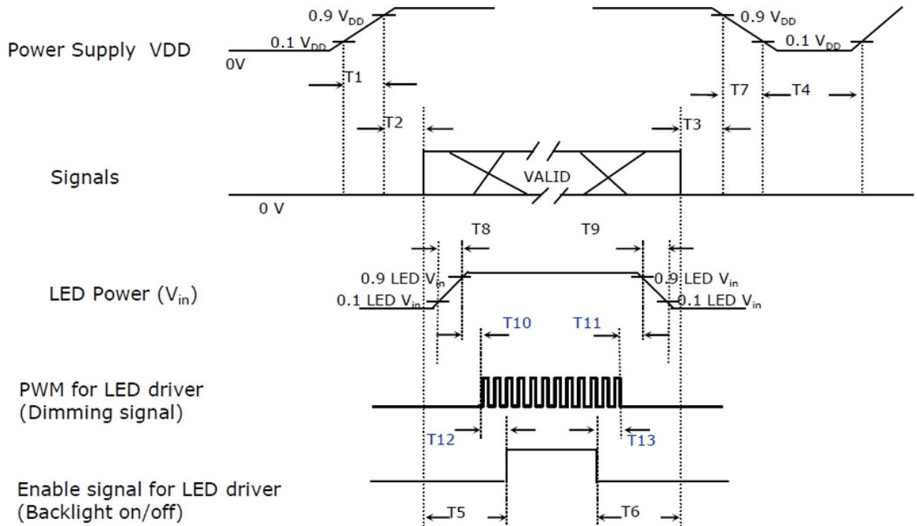
Figure 17 Power Sequence
