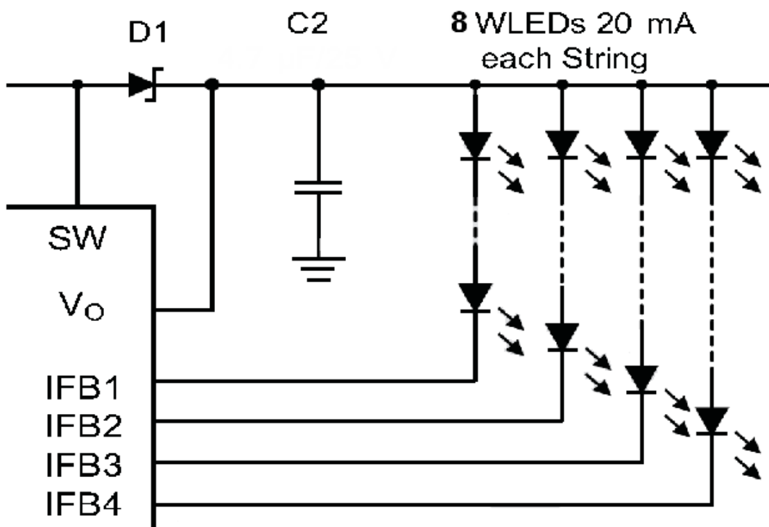
Figure 9 LED Circuit Diagram
