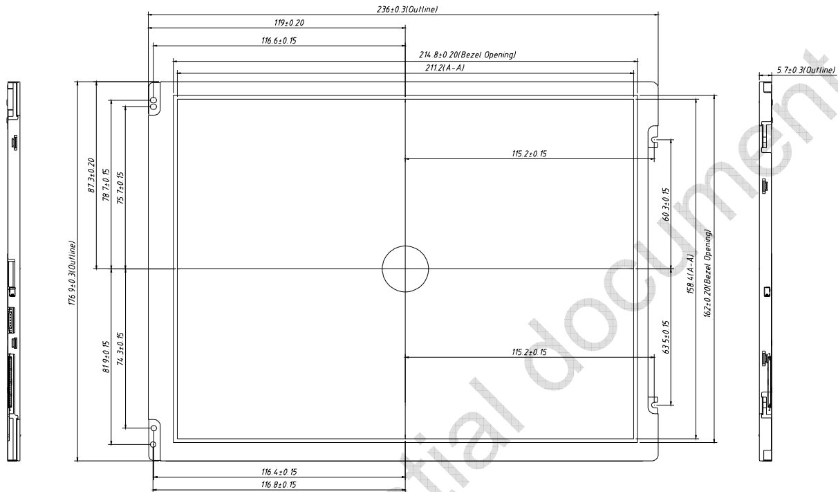
Figure 18 Reference Outline Drawing (Front Side)
