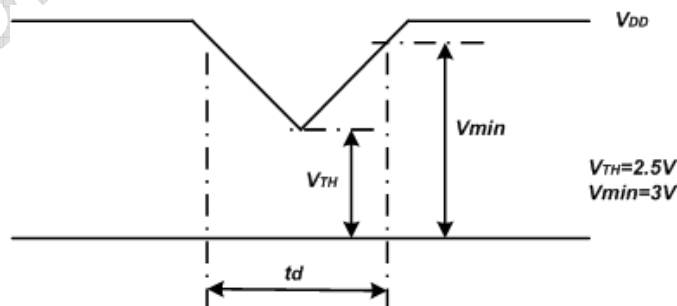
Figure 16 VDD Power Dip
