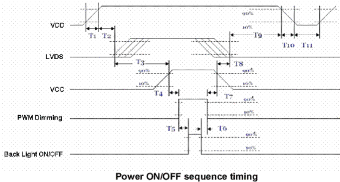
Figure 10 Power Sequence
