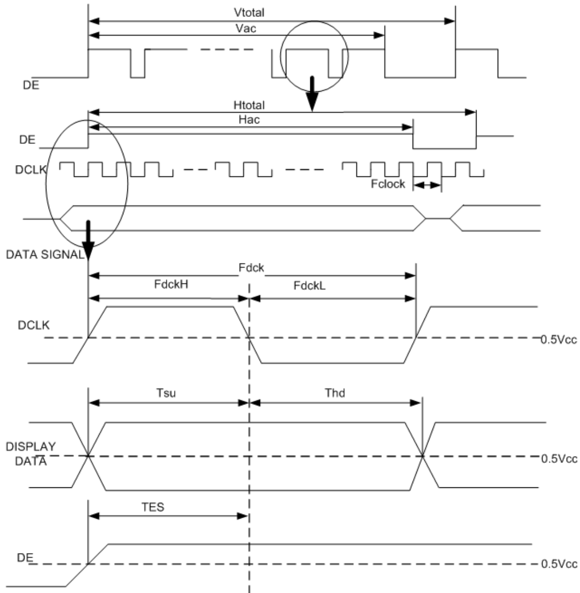
Figure 13 Timing Characteristics
