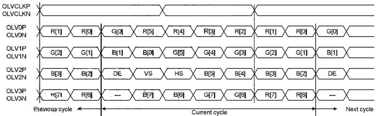
Figure 11 Data Mapping
