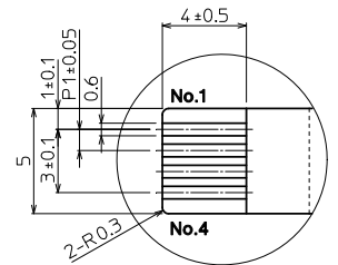
DETAIL B (5:1)
