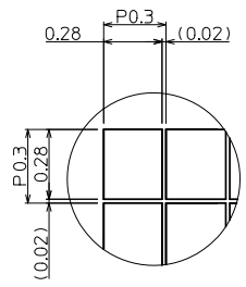
DETAIL A (NTS) (Dot Size)
