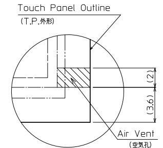
DETAIL E (5:1)
