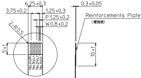
DETAIL D (2:1)
