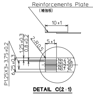
DETAIL C(2:1)
