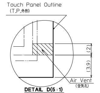
DETAIL D(5:1)
