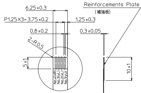
DETAIL E (2:1)
