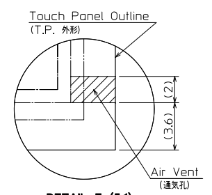
DETAIL F (5:1)
