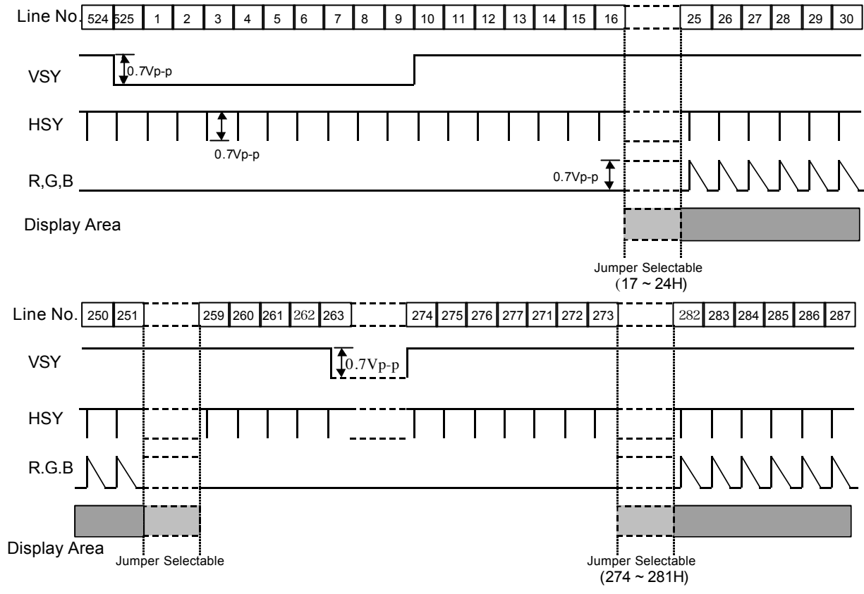
Fig.4-4 Vertical Timing (NTSC: Full/4:3mode)
