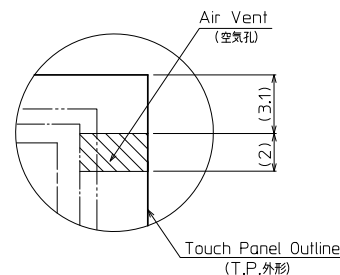
DETAIL D (5:1)
