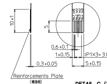
DETAIL C (2:1)
