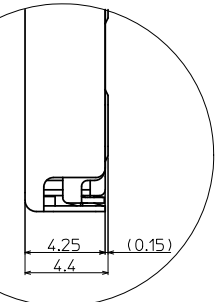
△ DETAIL B (5:1)
