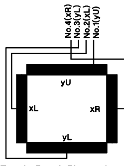
Touch Panel Pin-assign
