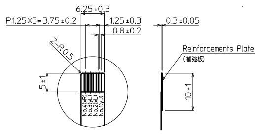
DETAIL C (2:1)
