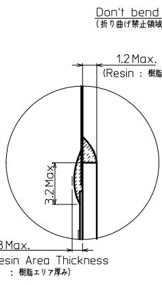
DETAIL D (5:1)
