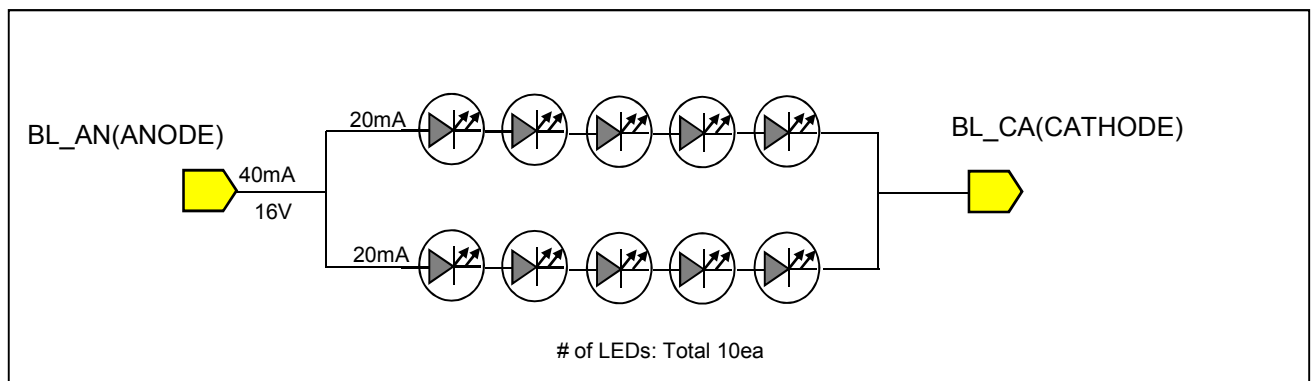
Fig 1. LED configuration
