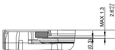
SECTION A-A SCALE 2/1
