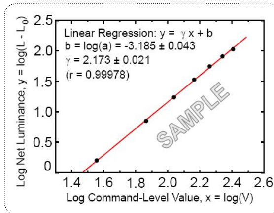
[Figure .13] Sample Log-log plot of luminance vs. gray scale
