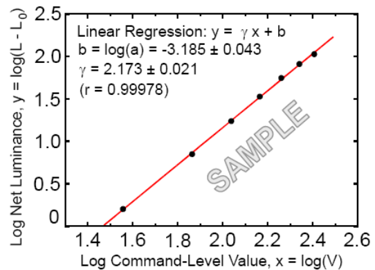
[ FIG 13 ] Sample Luminance vs. gray scale (using a 256 bit gray scale)
