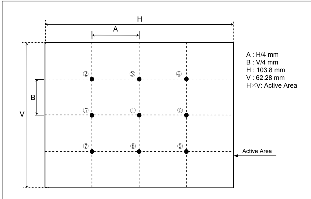
FIG. 2 Luminance
