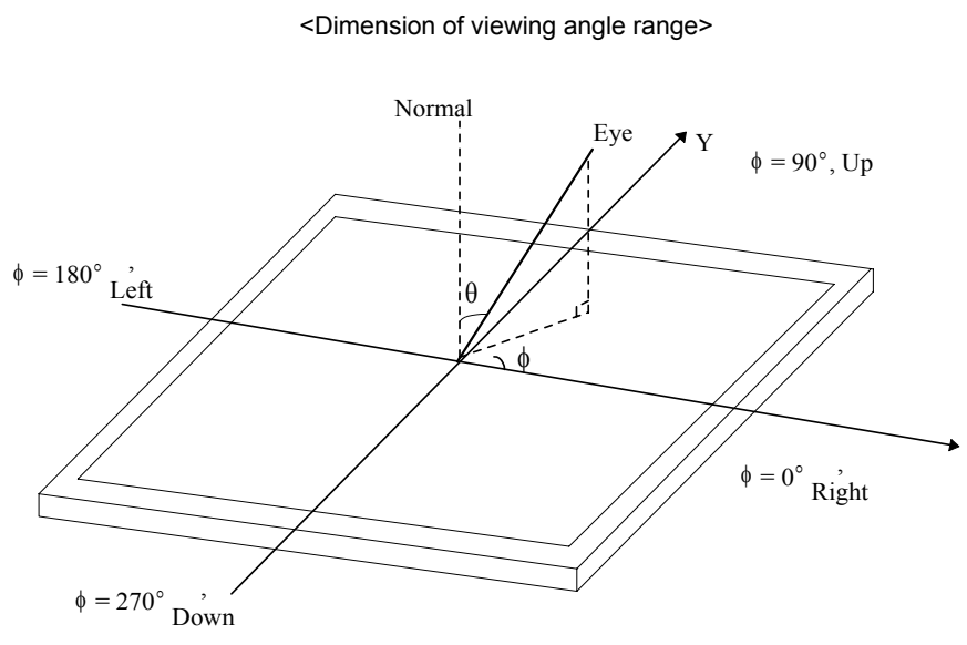
FIG. 4 Viewing angle
