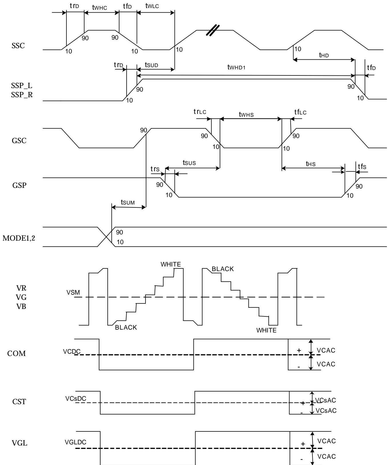
[FIG.4] Input Signal Timing Chart
