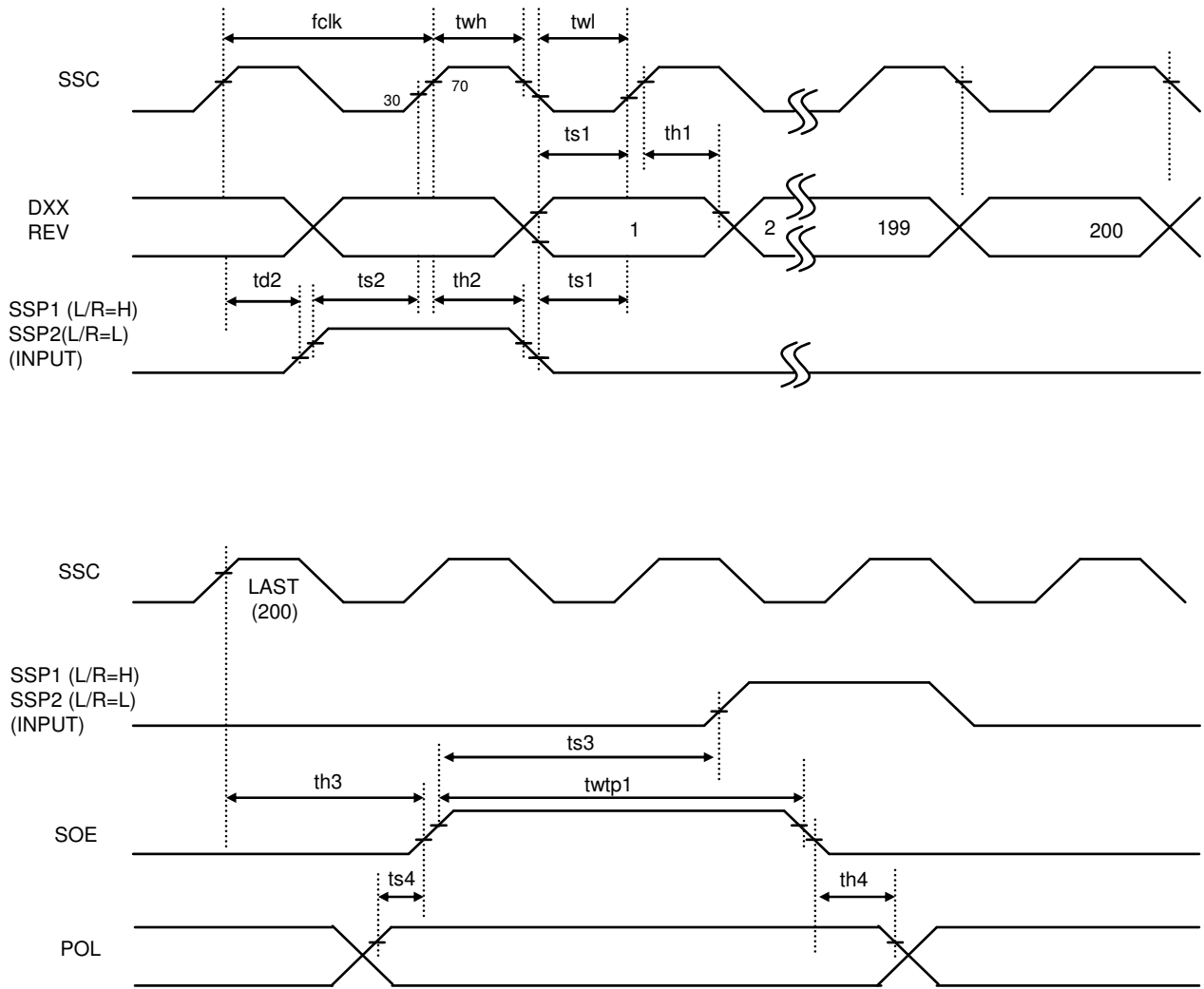
① Source D-IC Timing Diagram
