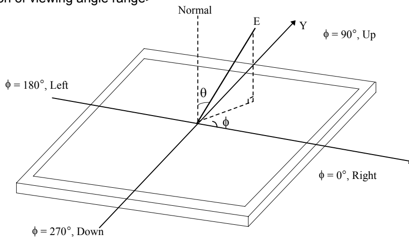
FIG. 4 Viewing angle
